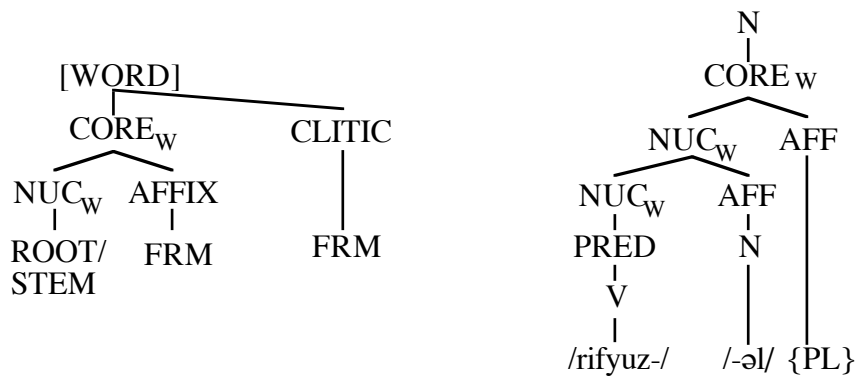
Figure 6: The layered structure of the word (template), the layered structure of refusals
