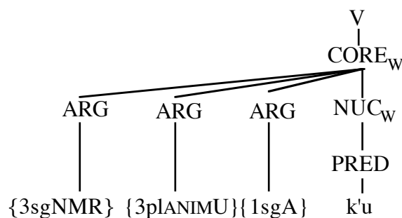
Figure 7: The layered structure of the word wičhák’u ‘I gave it to them’ in (2b) 29
